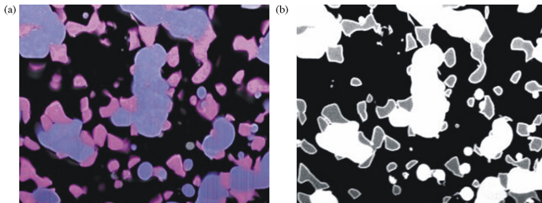
Fig. 3. (a) EDX and (b) SEM images matching for separation of three phases. Blue and red regions correspond to Ni and YSZ phases, respectively, in the EDX image.
