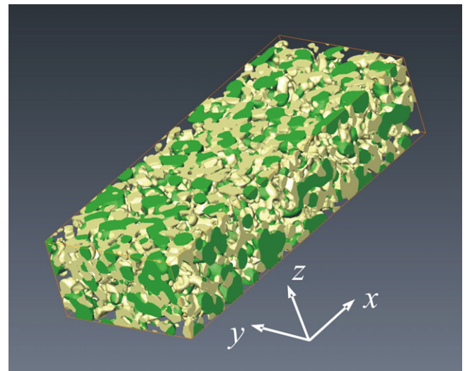
Fig. 4. Reconstructed Ni–YSZ anode microstructure ( 25.722 \mu\text{m} \times 11.624 \mu\text{m} \times 6.572 \mu\text{m} ; green: Ni, yellow: YSZ).
